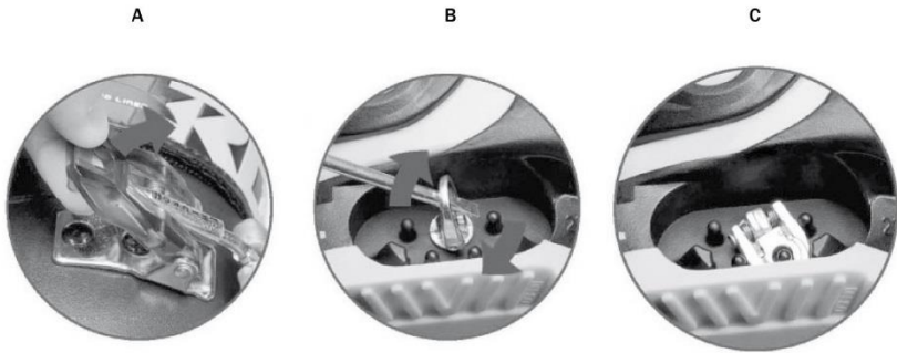
SAS - Size Adjustment System (Length Growth Compensator)
